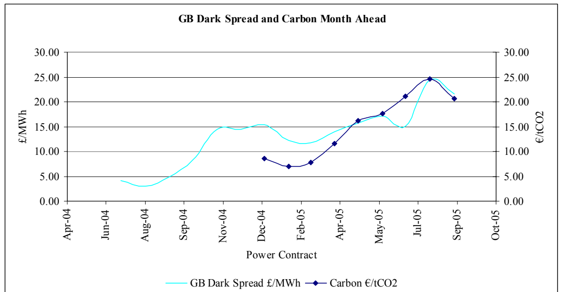
Figure 47 GB Month-Ahead Dark Spread Analysis 38
