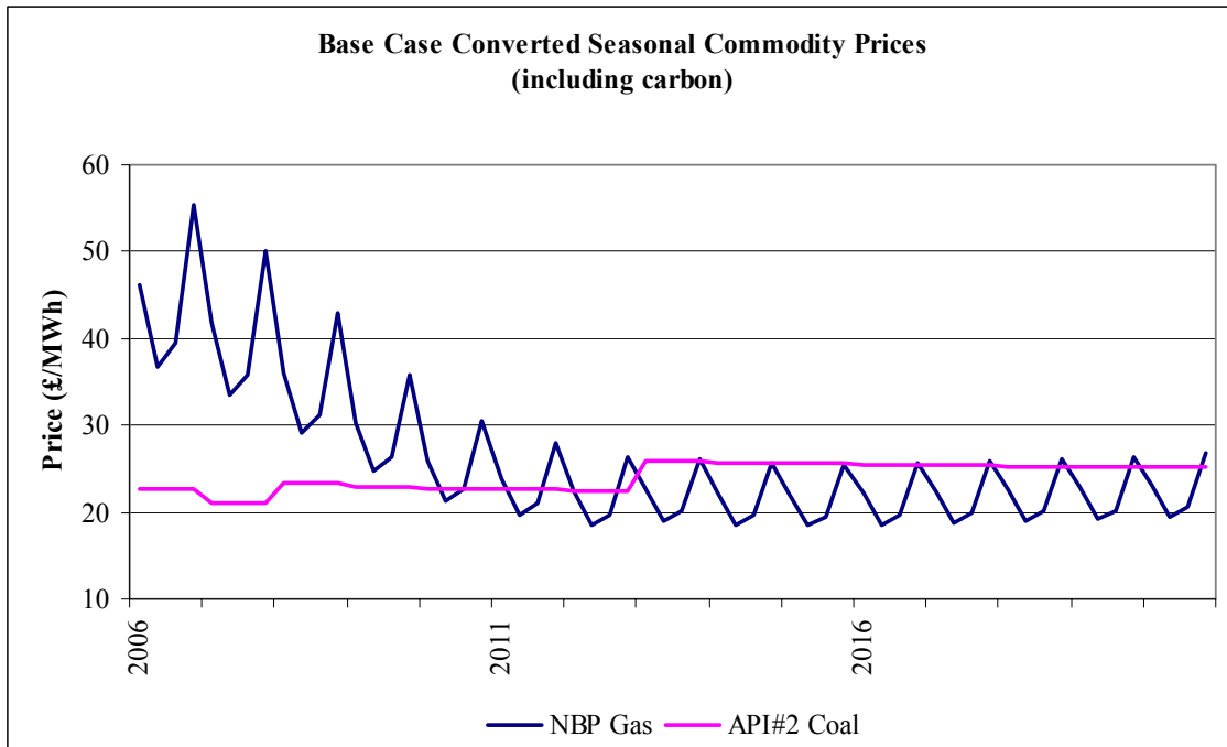
Figure 5: Base Case Converted Seasonal Commodity Prices (Including fuel costs and carbon costs at typical plant efficiencies)
