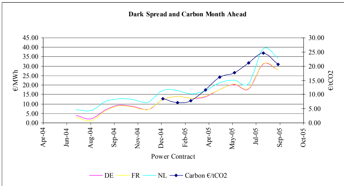
Figure 50: Month Ahead Dark Spread Analysis for Germany, France and Holland 41
