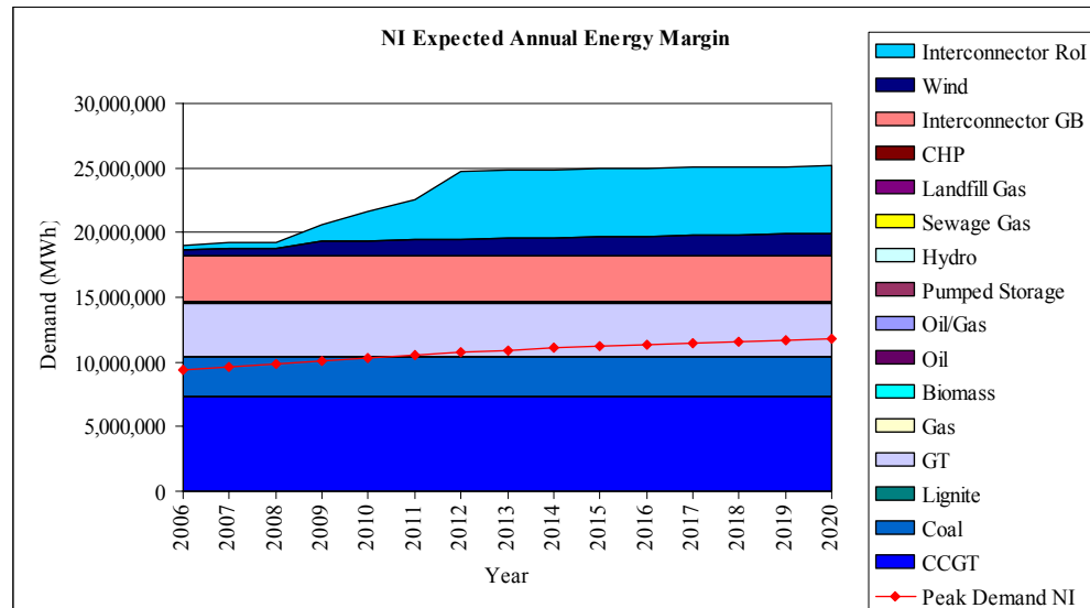
Figure 25: Northern Ireland Expected Annual Energy Margin
