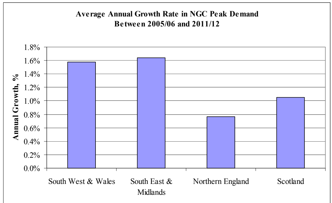
Figure 20: Locational Demand Growth 19
