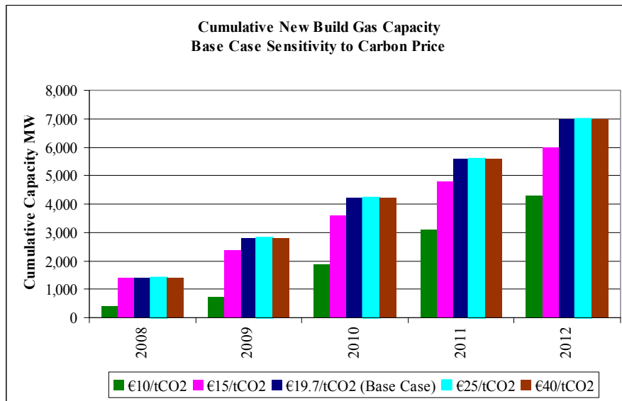
Figure 30: Impact of Phase II Carbon Prices on Capacity Build and Closures
