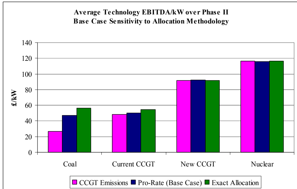
Figure 36: Impact of the Methodology of Power Sector Phase II Allocations on Generation Technology EBITDA
