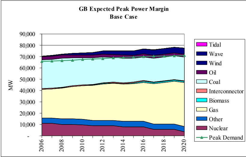
Figure 18: Expected Peak Power Margin
