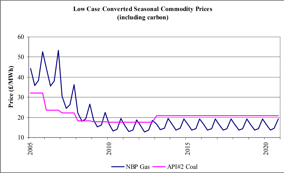
Figure 7: Low Case Converted Seasonal Commodity Prices (Including fuel costs and carbon costs at typical plant efficiencies)
