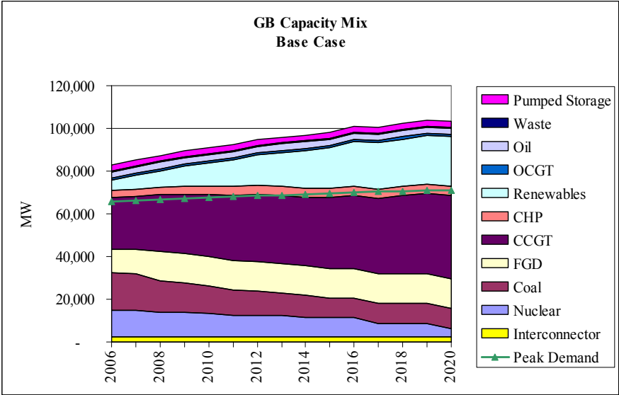
Figure 14: Base Case GB Capacity, Output and Emissions
