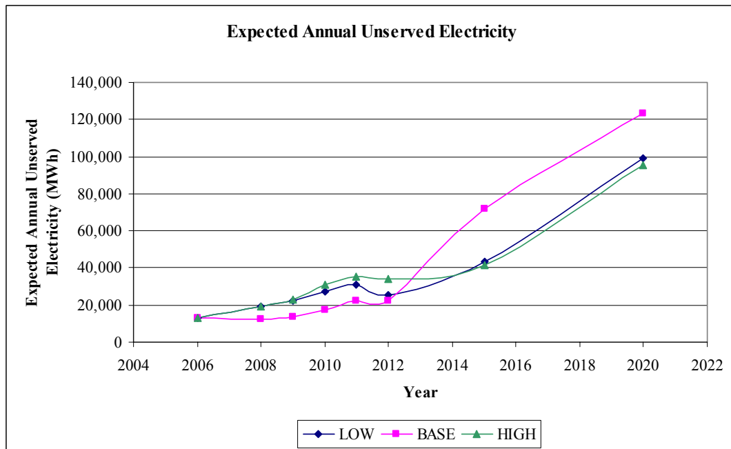
Figure 19: Expected Annual Unserved Electricity
