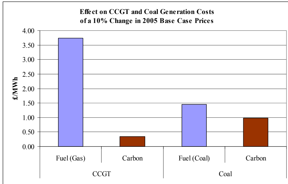
Figure 27: Sensitivity to a 10% Change in Carbon and Fuel Prices by Technology
