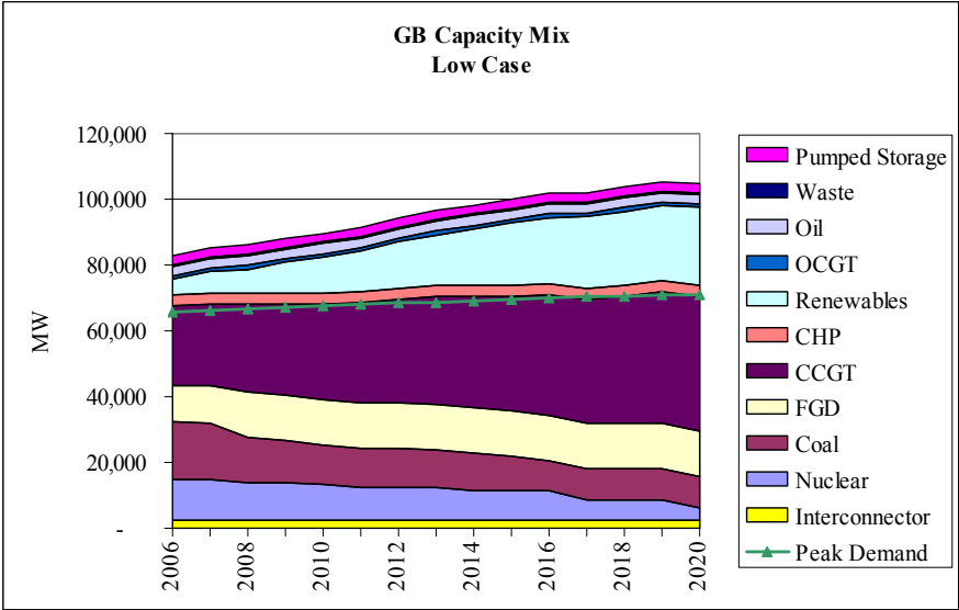
Figure 15: Low Case GB Capacity, Output and Emissions
