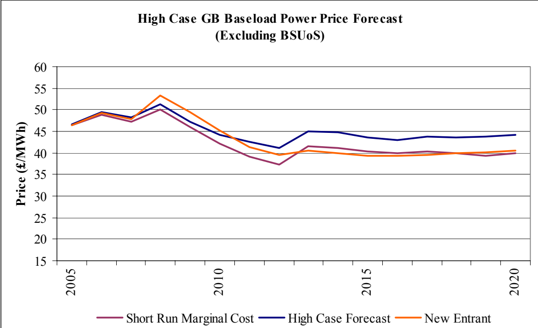
Figure 10: High Case GB Baseload Power Forecast (Excluding BSUoS)
