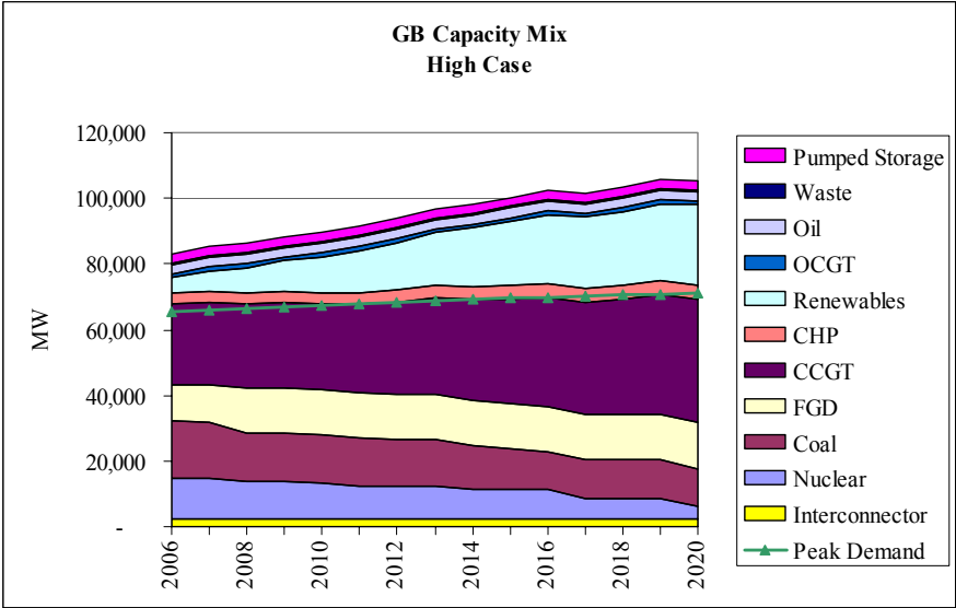
Figure 16: High Case GB Capacity, Output and Emissions
