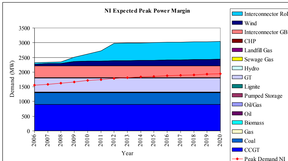
Figure 24: Northern Ireland Expected Peak Power Margin
