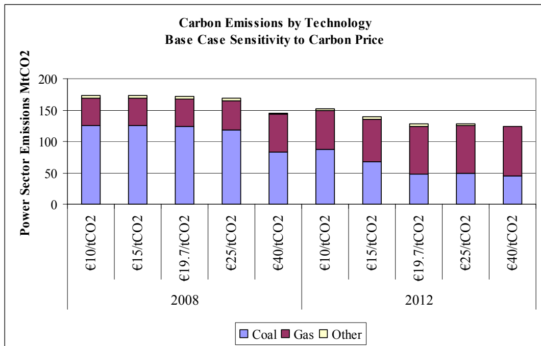
Figure 32: Impact of Phase II Carbon Prices on CO 2 Emissions by Technology 28
