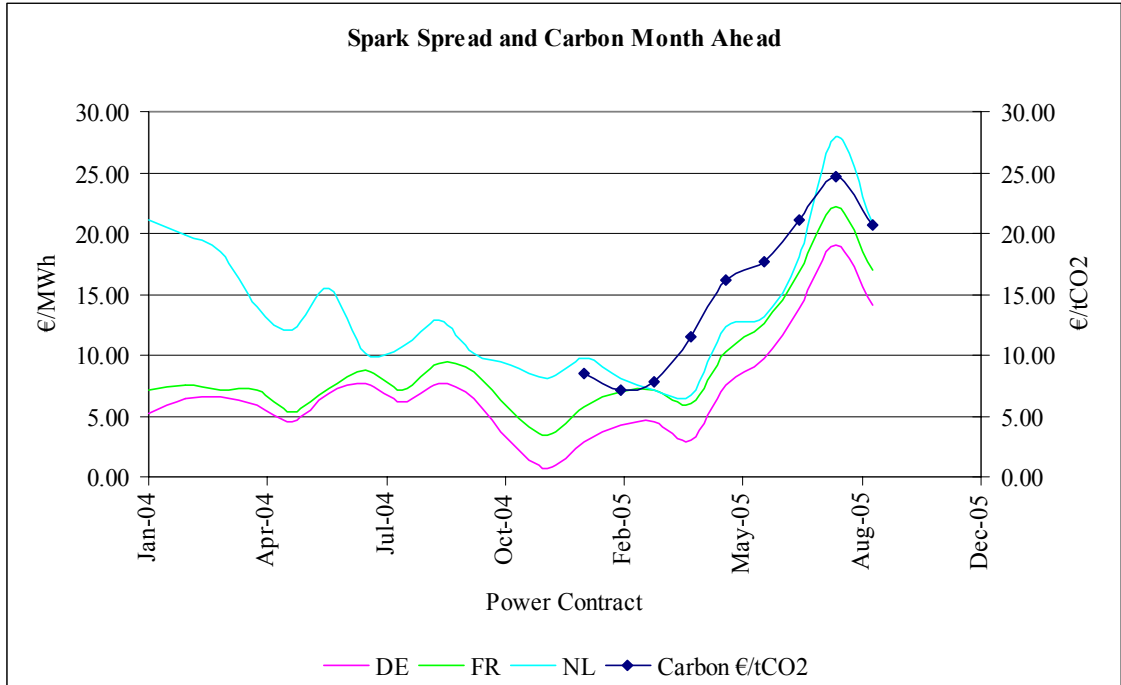
Figure 49: Month Ahead Spark Spread Analysis for Germany, France and Holland 40
