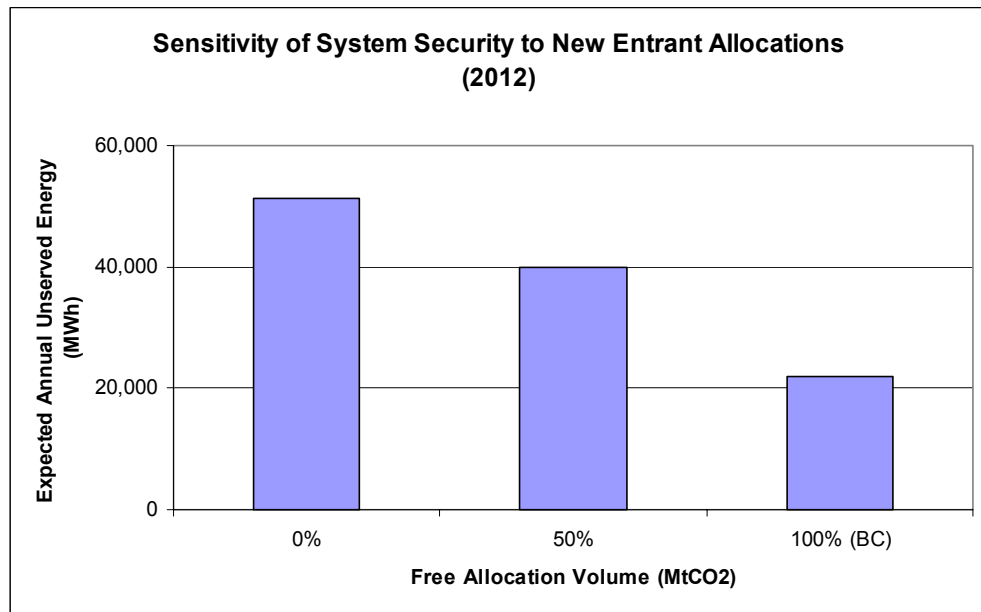
Figure 43: Sensitivity of System Security to New Entrant Allocations
