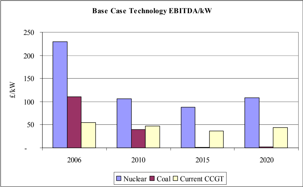
Figure 12: Profitability by Generation Technology
